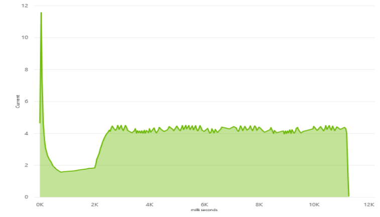
Obstruction in Point Motor
