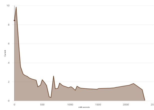
Carbon brush worn out
