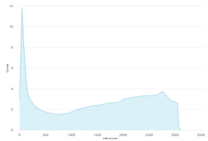
More friction due to lubrication problem
