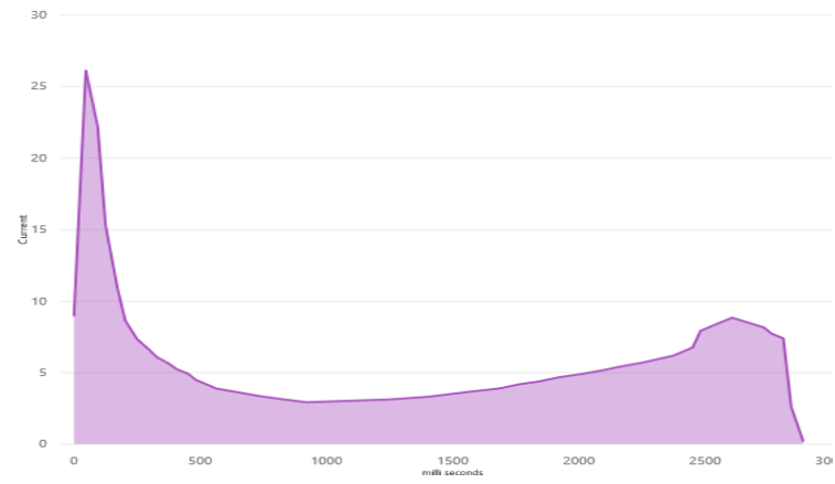
More current at locking time due to spring
